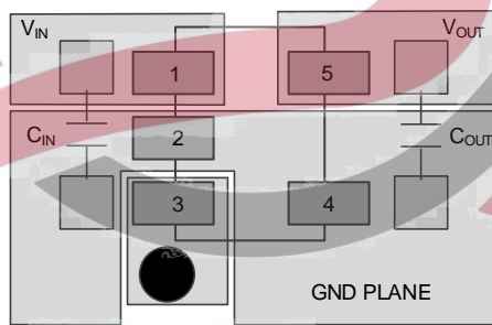
Figure 39. Layout Example for DBV Package
